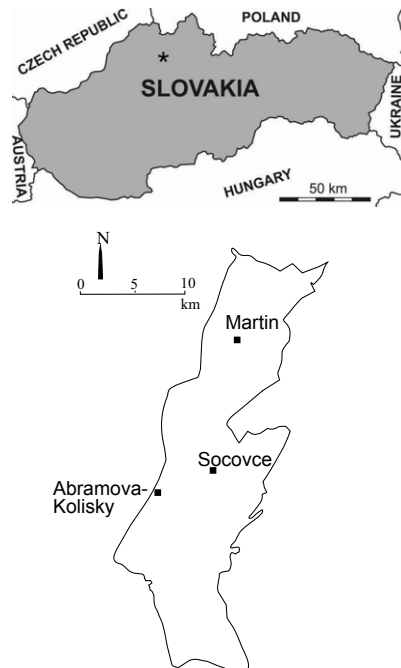
Fig. 1. Schematic map of the Turiec Basin in Slovakia with locations of the three sampling stops: Martin (49°03'52"N; 18°53'42"E), Socovce (48°57'11" N; 18°51'45"E) and Abramová-Kolísky (48° 55'47"N; 18°47'09"E).
