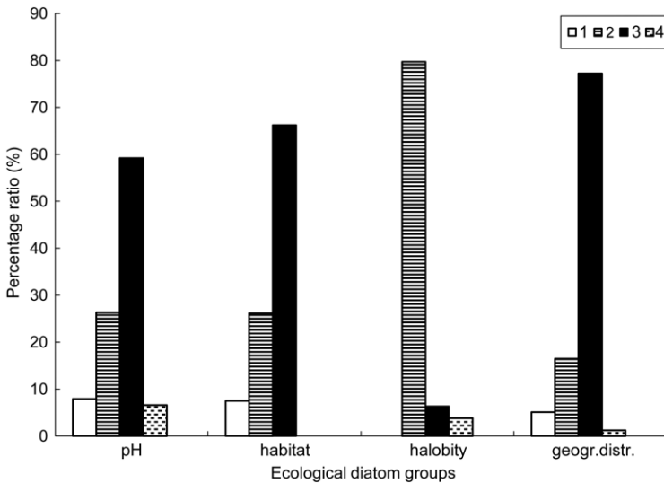
Fig. 3. Percentage ratio of the ecological groups diatoms. pH spectrum: 1 – acidophilic, 2 – indifferent, 3 – alkaliphilic, 4 – alkalibiontic; »Habitat« spectrum: 1 – planktonic, 2 – periphytic (deep water forms), 3 – periphytic (epiphytic); Halobion spectrum: 1 – halophobous, 2 – indifferent, 3 – halophilous; Geographical distribution: 1 – tropical forms, 2 – boreal forms, 3 – cosmopolitans, 4 – north-alpine forms.
