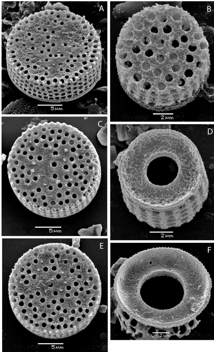
Fig. 6. Alveolophora jouseana (Moiss.) Moiss., scanning electron microscope images (A–F): external valvae face view (A–B, C, E), internal view of valve showing the Ringleiste (D, F).
