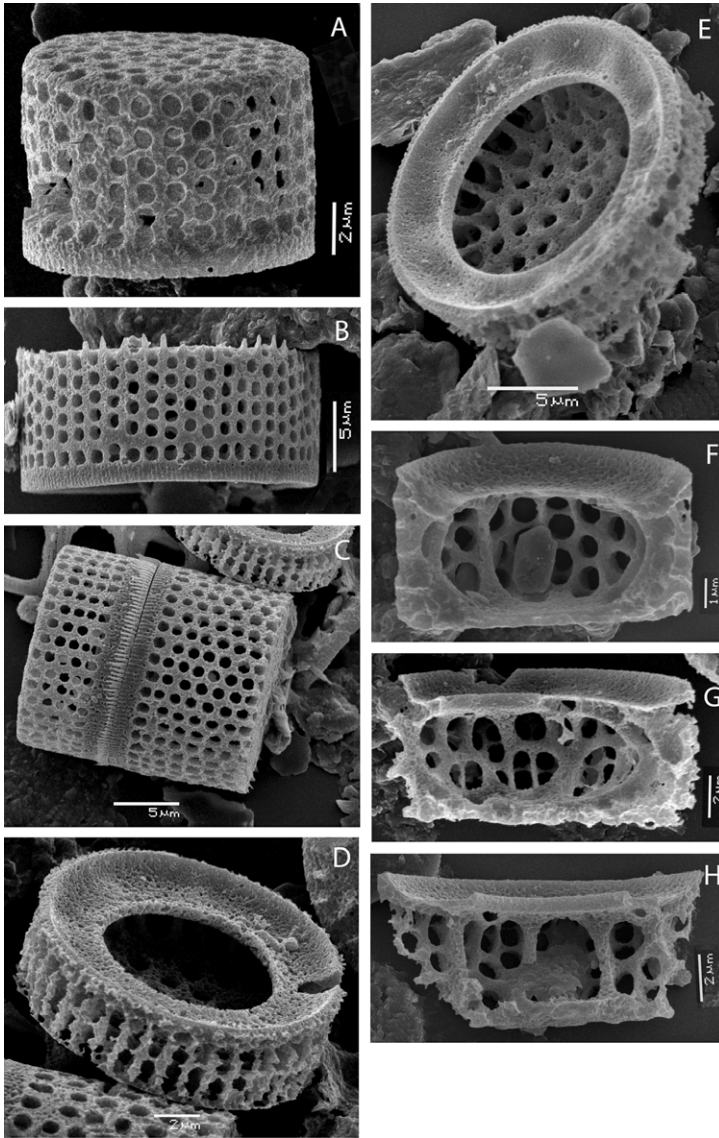
Fig. 7. Alveolophora jouseana (Moiss.) Moiss., scanning electron microscope images (A–H): external view of mantle (A, C), external view of mantle showing separating spines (B), internal view of valvae showing the Ringleiste (E), internal view showing valve with costae (F–H).
