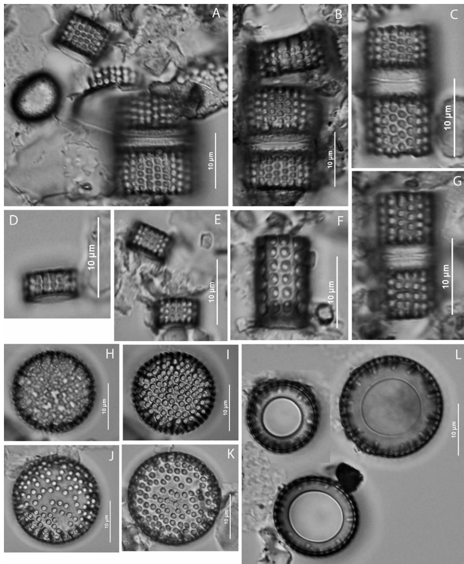
Fig. 5. Alveolophora jouseana (Moiss.) Moiss., light microscope images (A–L): external view of mantle (A–G), external view of valve face showing areolae position (H–K), external view of valve from the Ringleiste with channels of rimoportulae (L).
