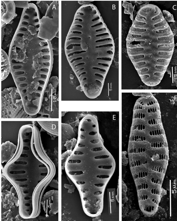
Fig. 10. Scanning electron microscope images (A–F): Staurosirella sp. 1, internal valve view (A–B), Staurosirella sp. 1, external valve view (C), Staurosirella leptostauron (Ehr.) Williams et Round, internal valve view (D–E), Staurosirella martyi (Héríb.) Morales et Manoylov (F).
