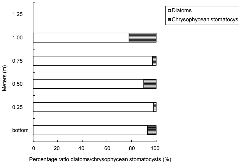
Fig. 4. Percentage ratio of the diatom frustules/chrysophycean stomatocysts.
