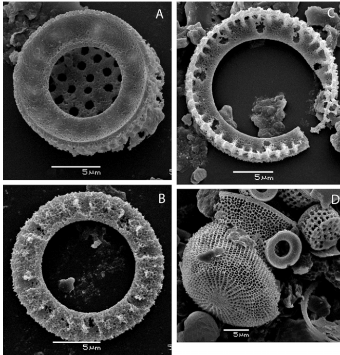
Fig. 8. Scanning electron microscope images (A–D): Alveolophora jouseana (Moiss.) Moiss., internal valve view showing different stages of dissolved Ringleiste (A–C), Melosira undulata (Ehr.) Kütz., external valve view (D).
